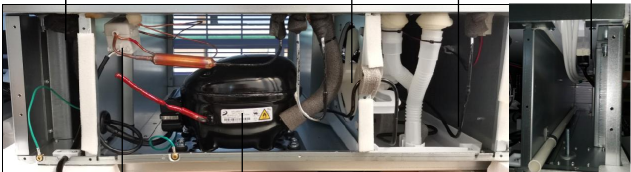
Control board repair from the lower right of the front
