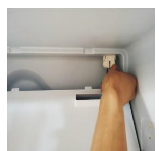
4. Unplug the terminal block and remove the cover plate
